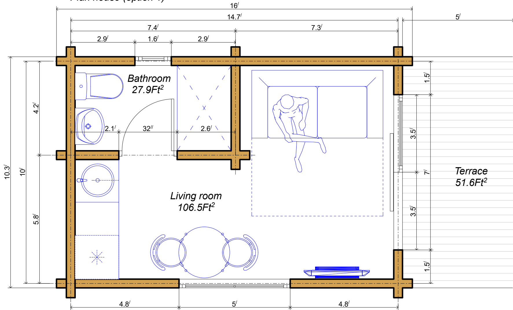
Plan house (option 1)
